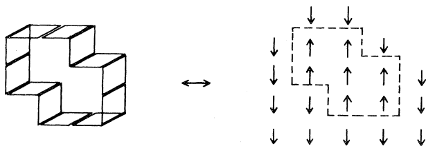
FIG. 31. A two-dimensional slice of a block of flipped spins in the three-dimensional Ising model and its corresponding graph in the Ising gauge model.
