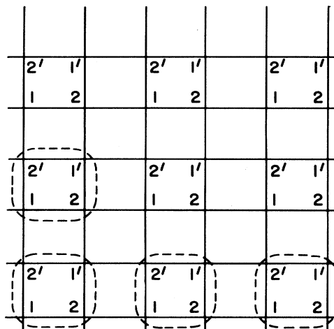
FIG. 67. Sites, blocks, and degrees of freedom for staggered Euclidean fermions.
