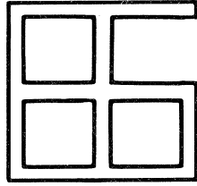
FIG. 24. Same as Fig. 23 after one-link variable integration.
