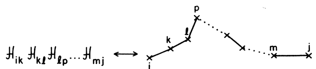
FIG. 70. A pictorial representation of the matrix inversion method of Von Neumann and Ulam.
