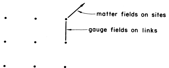
FIG. 48. The lattice degrees of freedom of the two-dimensional electro-dynamics of the planar model. The variables \Theta(r) reside on sites, and the gauge fields are on links.
