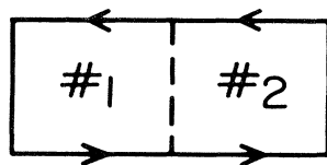
FIG. 56. A six-link rectangular loop as a probe for “thick” strings.
