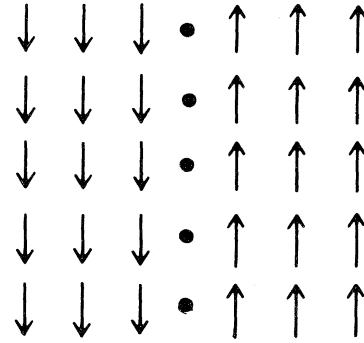
FIG. 32. A low-temperature planar interface in an Ising model.
